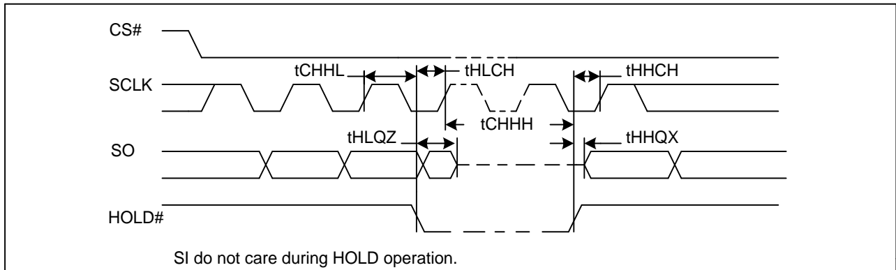
Figure46. Hold Timing
