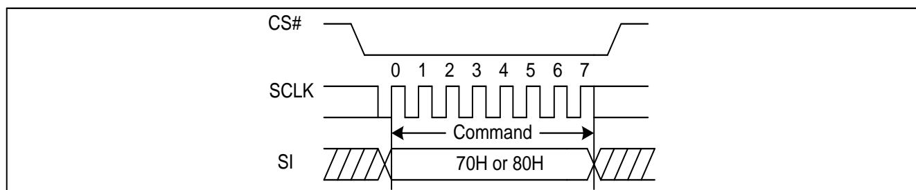
Figure23. Enable/Disable SO to Output RY/BY# Diagram
