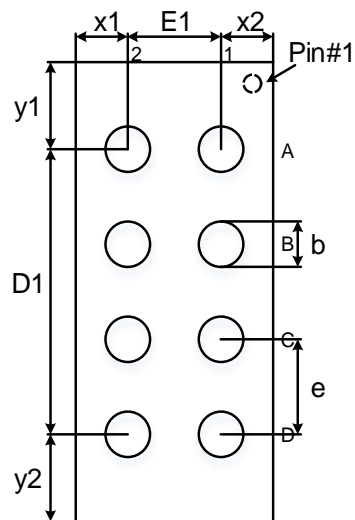
BOTTOM VIEW (BALL SIDE)
