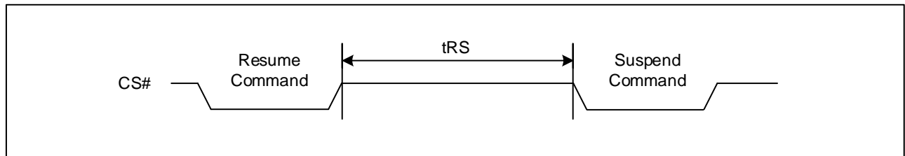
Figure43. Resume to Suspend Timing Diagram
