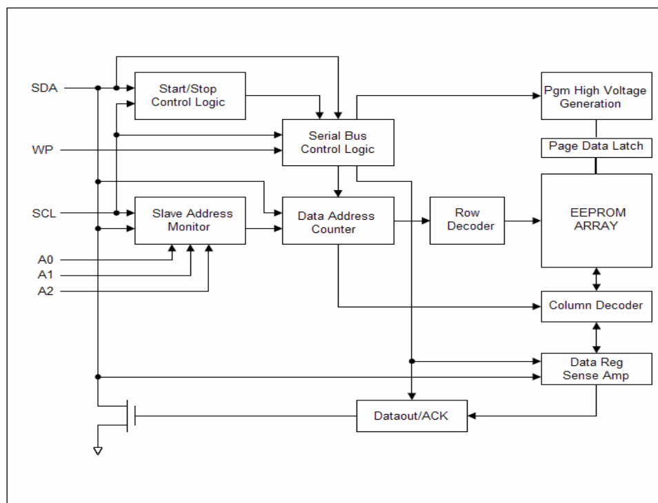
Block Diagram
