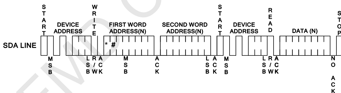
Figure 7: Random Read
