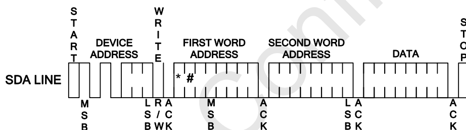
Figure 3: Byte Write
