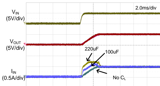
Inrush Current Response
