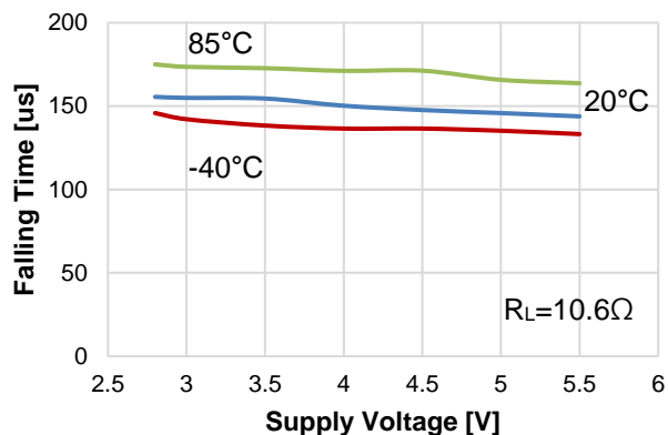
Falling Time vs. Supply Voltage
