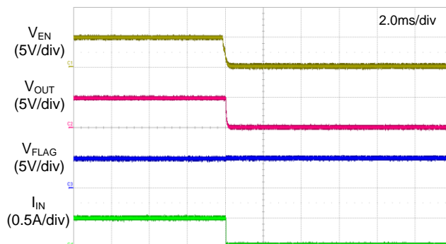
Turn OFF
