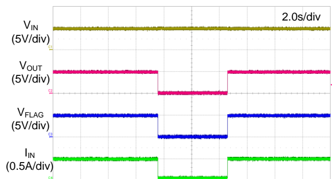
Thermal Shutdown
