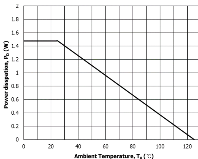
Power Dissipation( P_D ) vs. Ambient Temperature( T_A )
