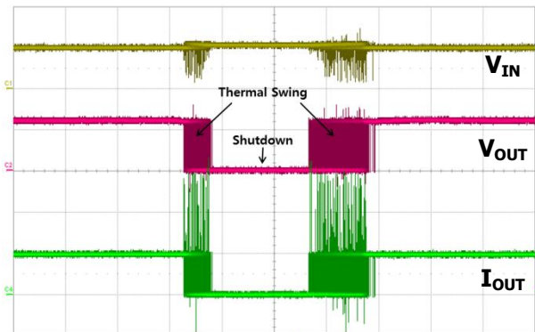
- V_{IN} : 2.0V/div, V_{OUT} : 1.0V/div, I_{OUT} : 2A/div, 5.0s/div Thermal Shutdown & Recovery ( C_{SS}=470pF , R1=R2=10k\Omega , V_{IN}=2.0V , V_{EN}=V_{BIAS}=5.0V )
