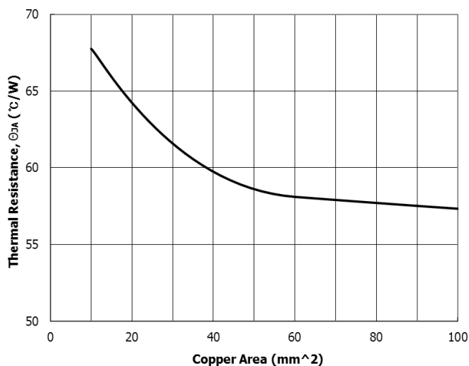
Thermal Resistance( \theta_{JA} ) vs. Copper Area
