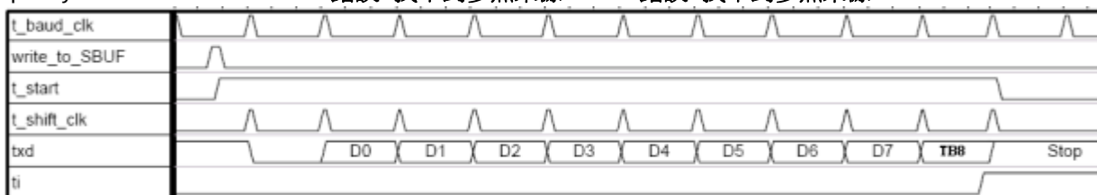
Fig. 8-5: Transmit modes 2 and 3
