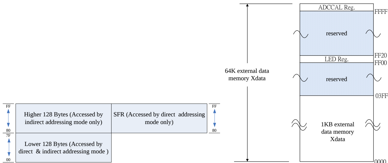
Fig. 3-2: RAM architecture
