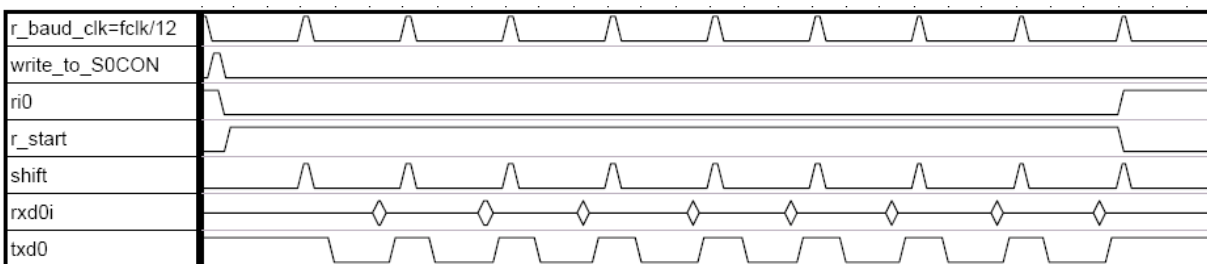
Fig. 8-2: Receive mode 0
