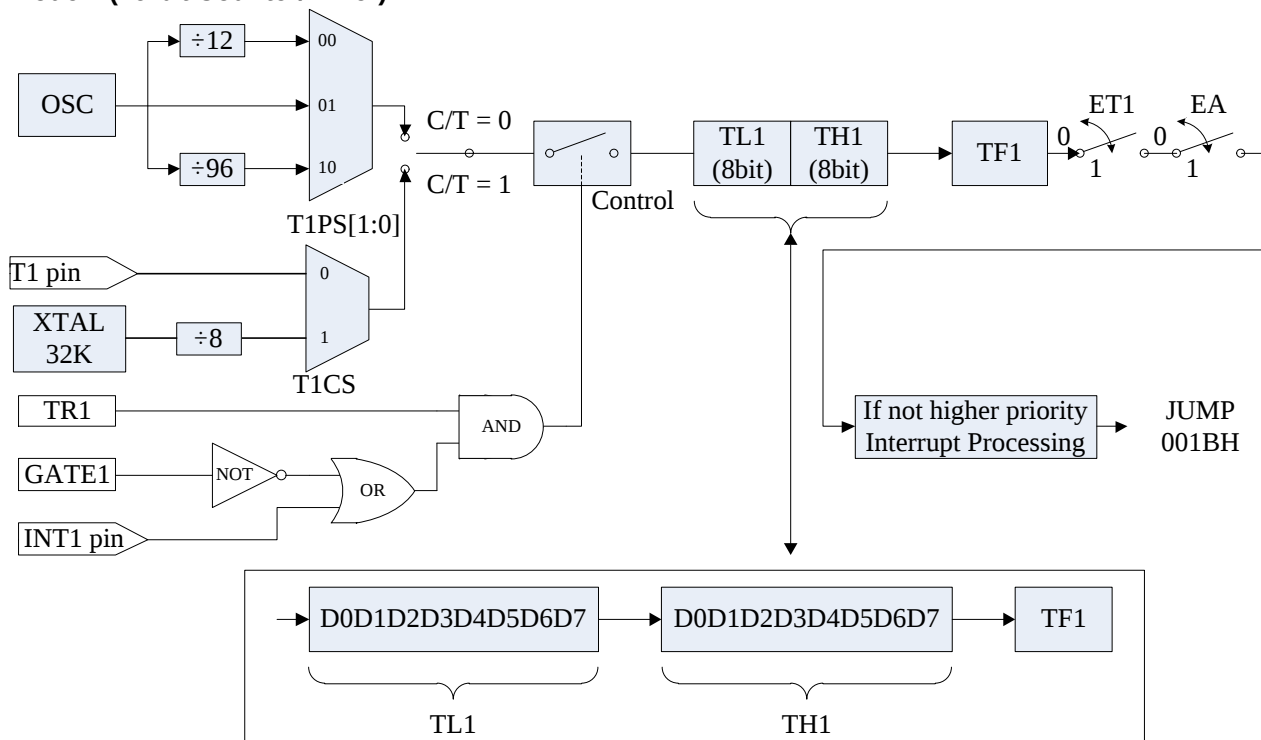
Fig. 6-2: Mode 1 16 bit Counter/Timer operation
