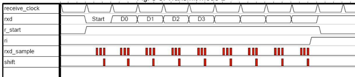
Fig. 8-4: Receive mode 1
