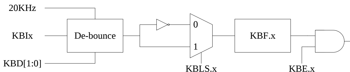
Figure 18-2 keyboard input circuitry
