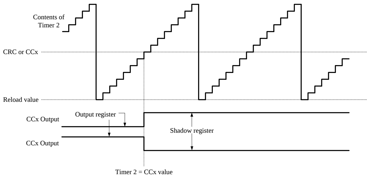
Fig. 7-6: Compare mode 1 function
