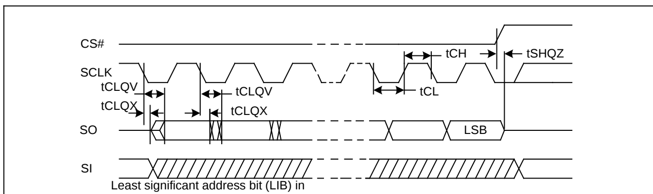
Figure27. Output Timing
