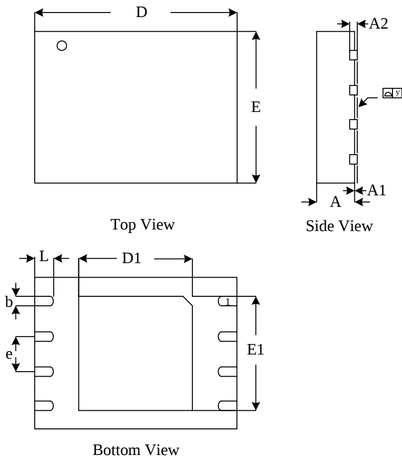
Figure30. WSON8 (6*8mm)
