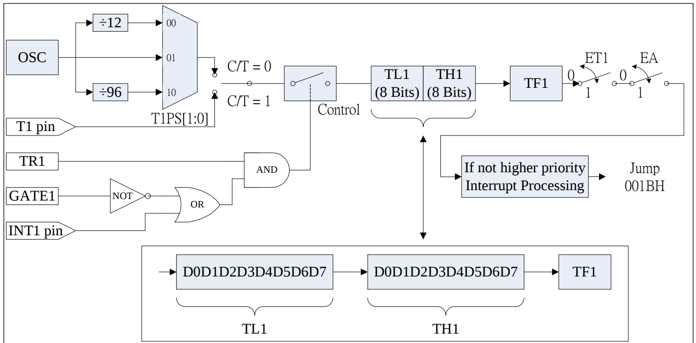
Fig. 7-1: Mode 1 16 bit Counter/Timer operation
