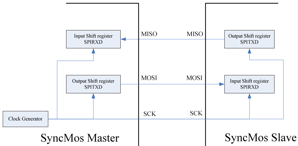
Fig. 15-2: SPI Master and slave transfer method
