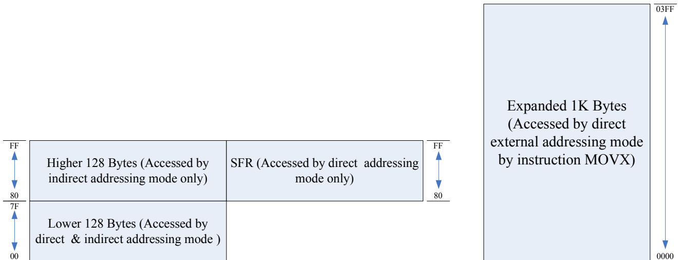
Fig. 3-2: RAM architecture
