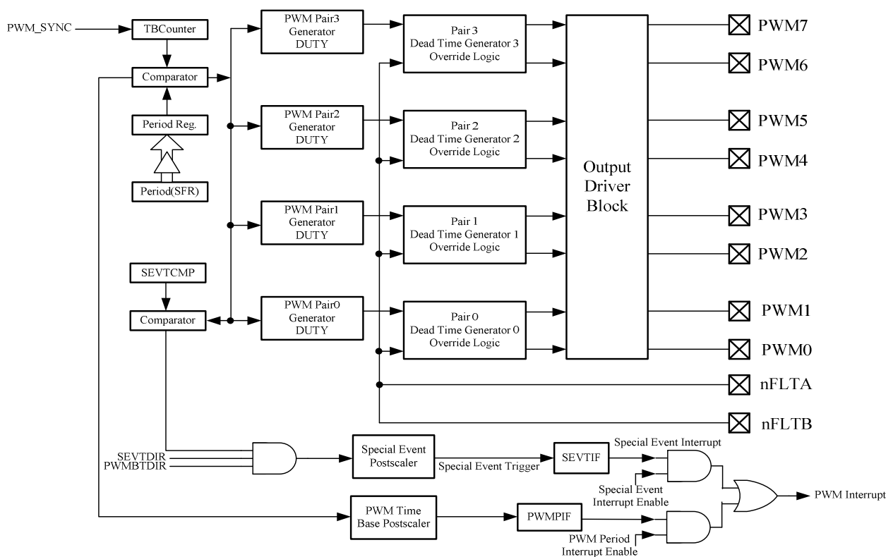
Fig. 13-1: Working module of the PWM
