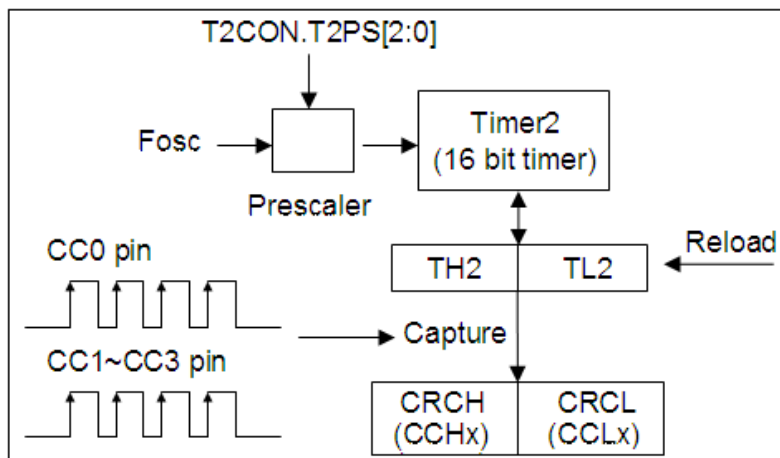
Fig. 8-7: Capture mode 0 function
