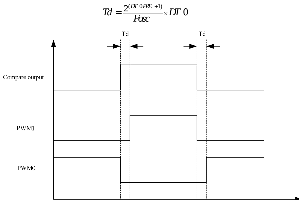
Fig. 13-3: PWM output Compare
