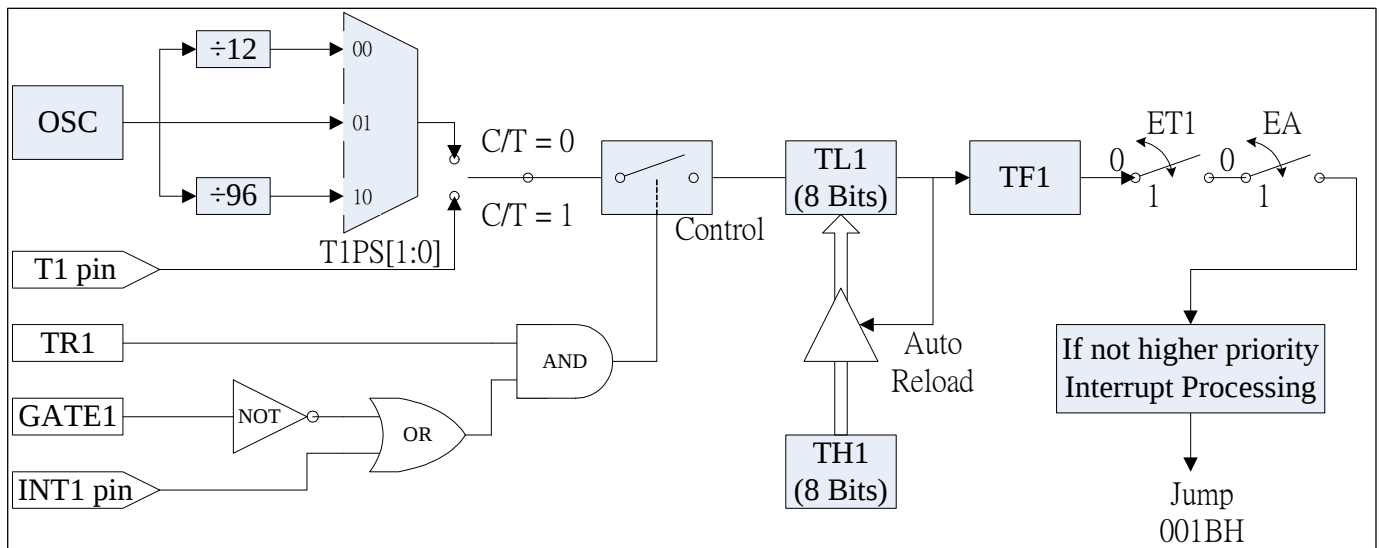
Fig. 7-2: Mode 2 8-bit auto-reload Counter/Timer operation.
