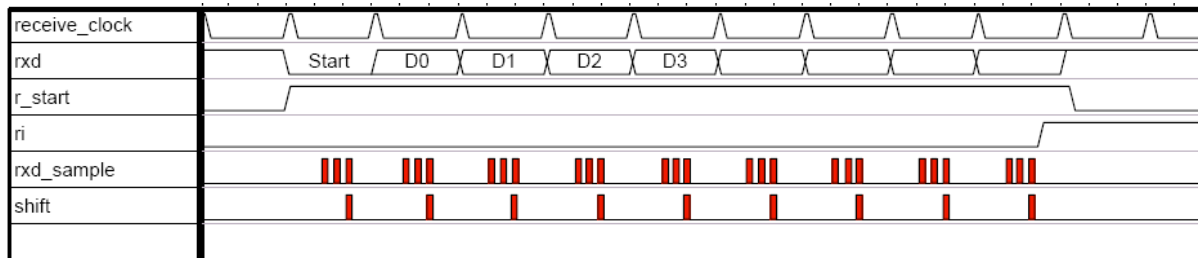
Fig. 9-4: Receive mode 1
