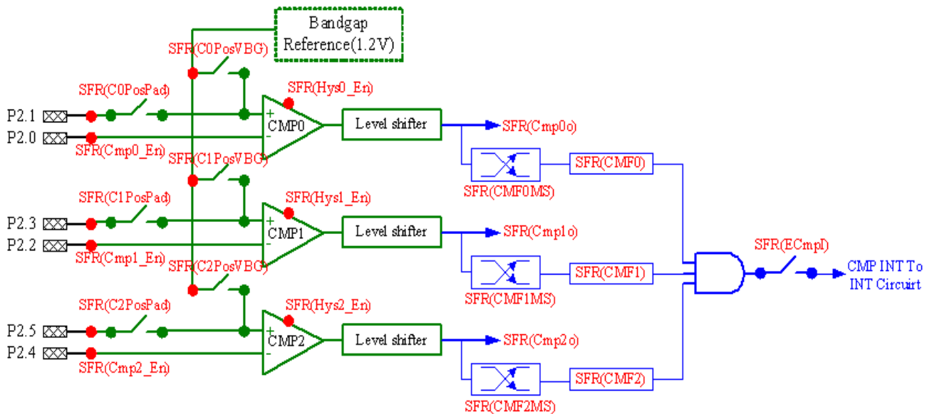
Fig. 19-1: Operation of Comparator Mode
