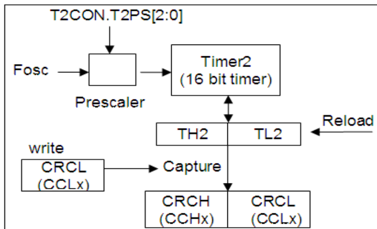
Fig. 8-8: Capture mode 1 function
