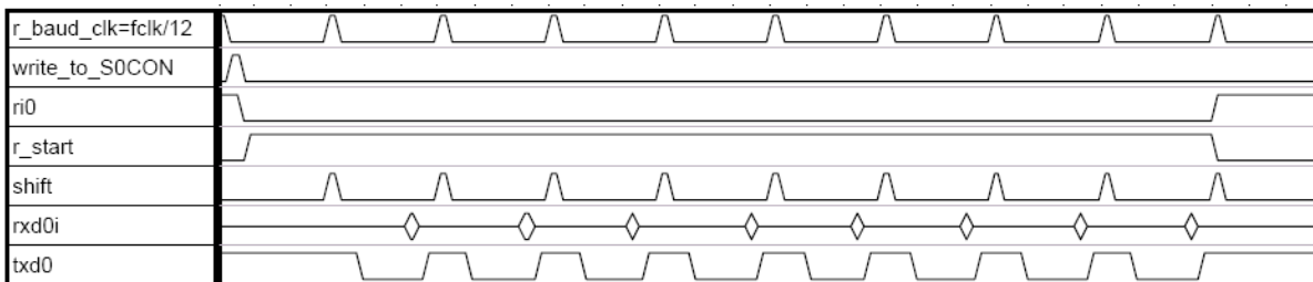
Fig. 9-2: Receive mode 0
