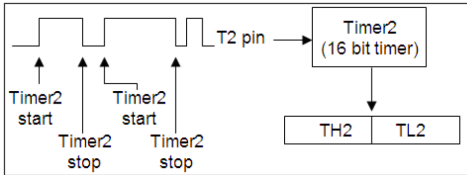
Fig. 8-3: Gated timer mode function
