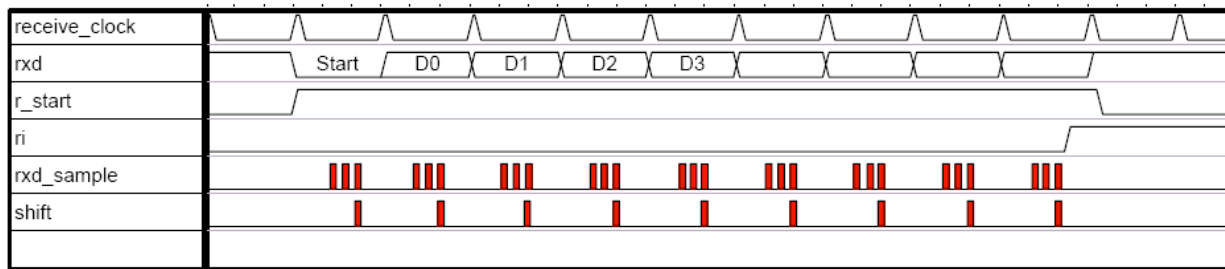
Fig. 7-4: Receive mode 1
