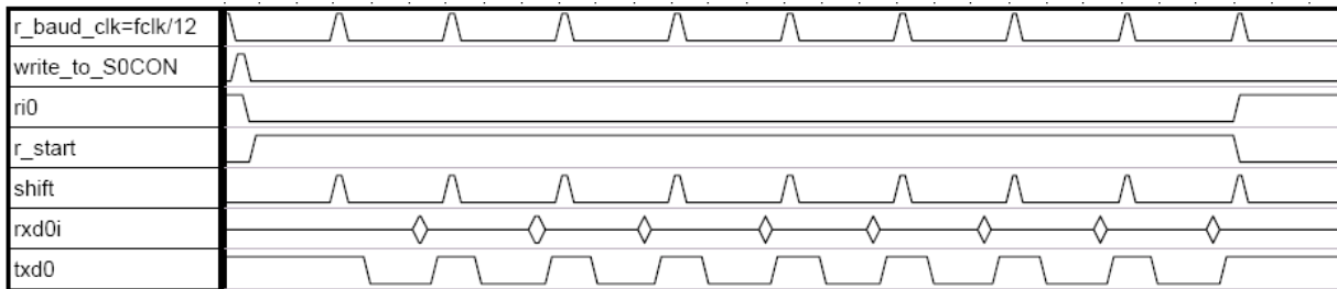
Fig. 7-2: Receive mode 0
