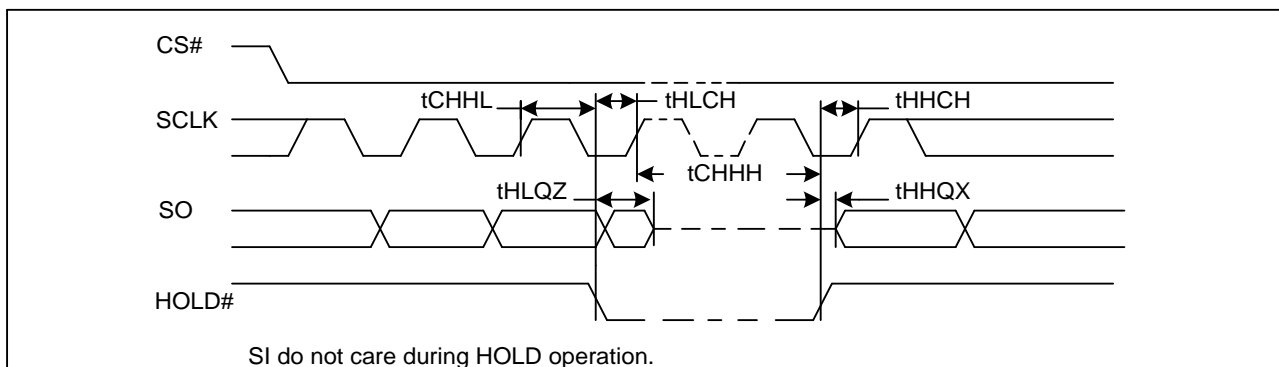
Figure49. Hold Timing
