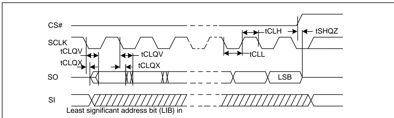
Figure47. Output Timing
