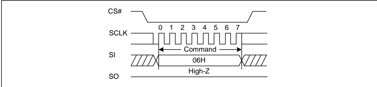
Figure4. Write Enable Sequence Diagram
