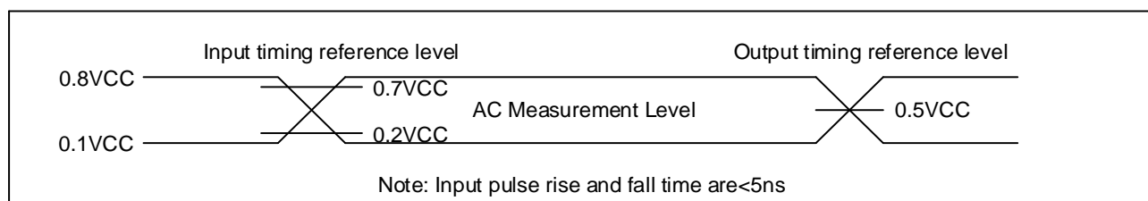
Figure45. Input Test Waveform and Measurement Level
