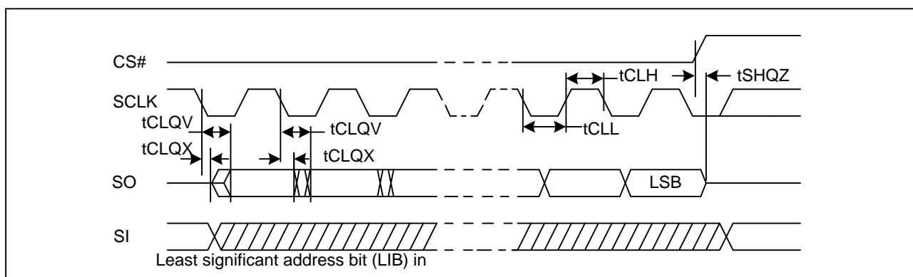
Figure44. Output Timing
