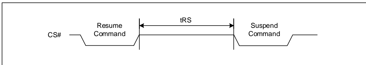
Figure45. Resume to Suspend Timing
