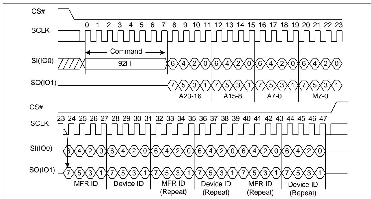
Figure 29. Dual I/O Read Manufacture ID/ Device ID Sequence Diagram
