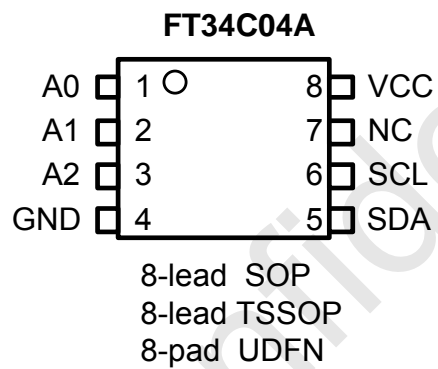
Figure 1: Package types
