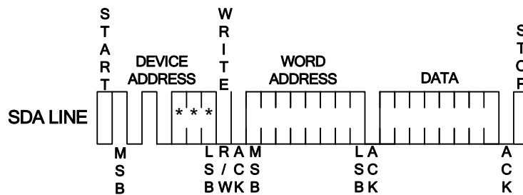
Figure 5: Byte Write
