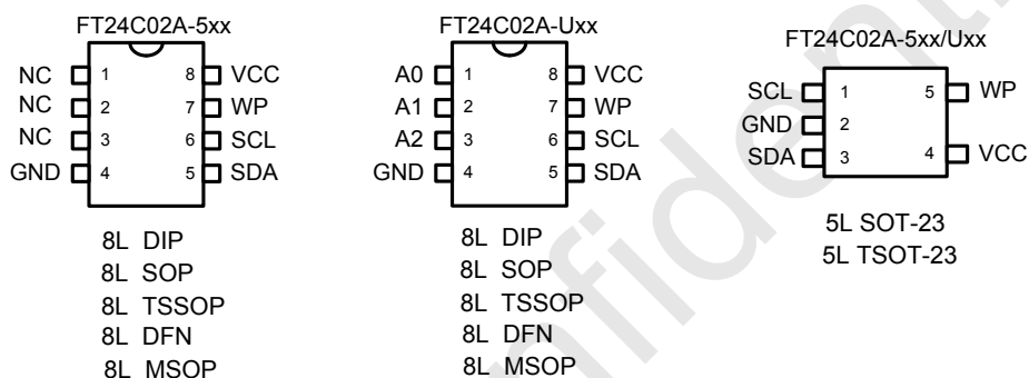
Figure 1: Package types
