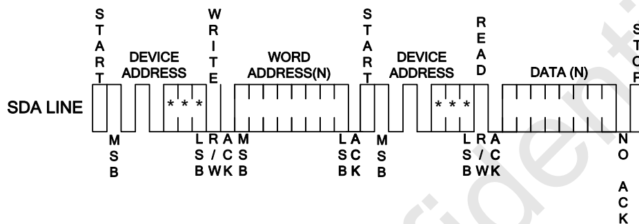
Figure 9: Random Read
