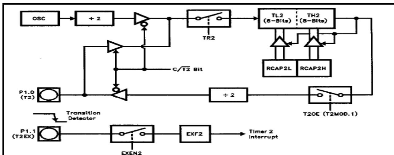
Fig. 7-4 : Timer 2 in clock-out mode
