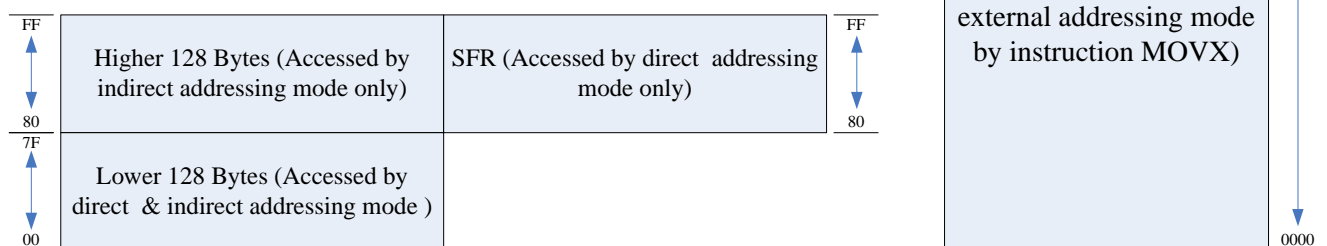
Fig. 3-2: RAM architecture
