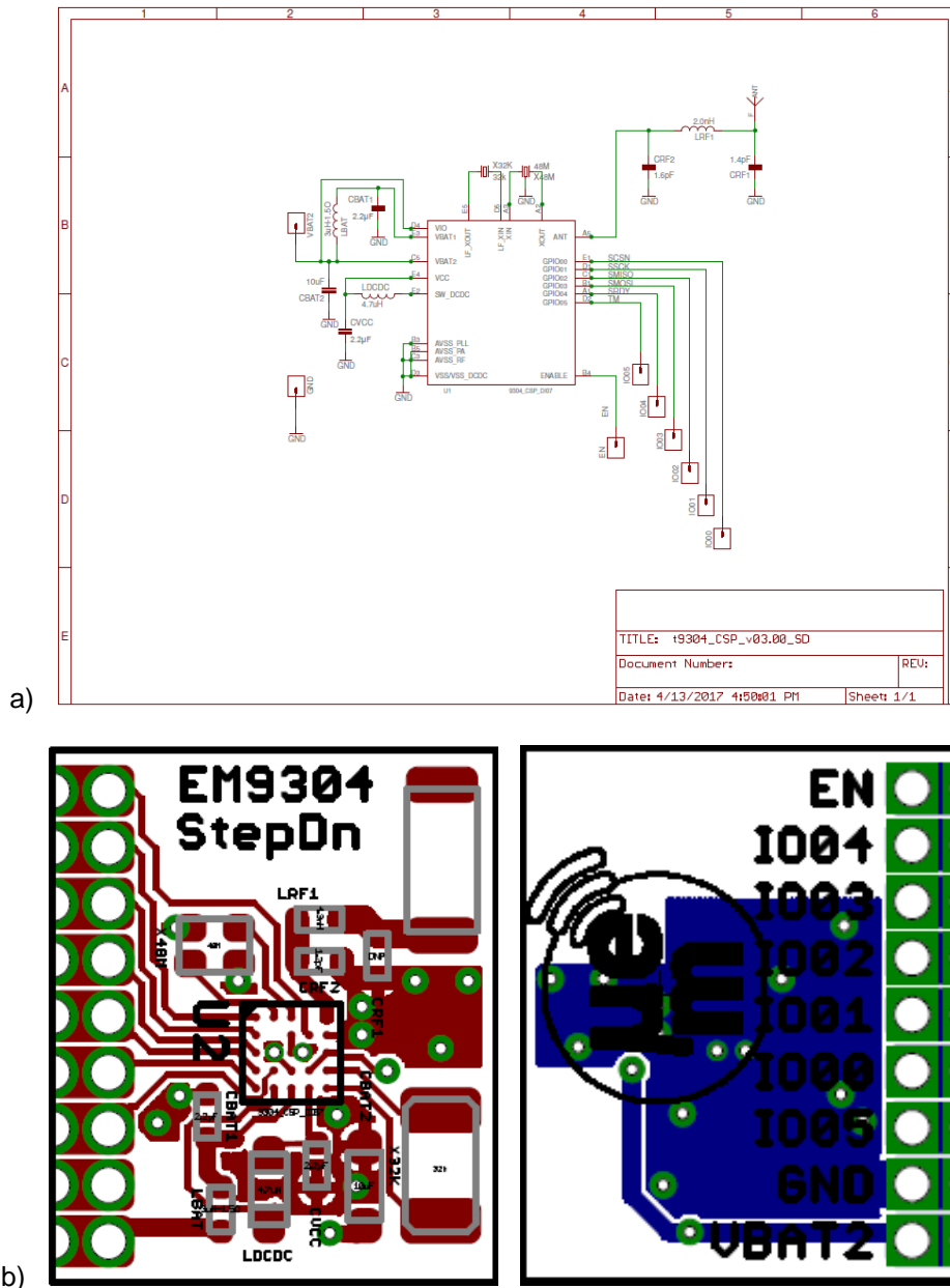
Figure 8: WLCSP DCDC Step-Down Configuration a) Schematic; b) Layout (Top, Bottom)
