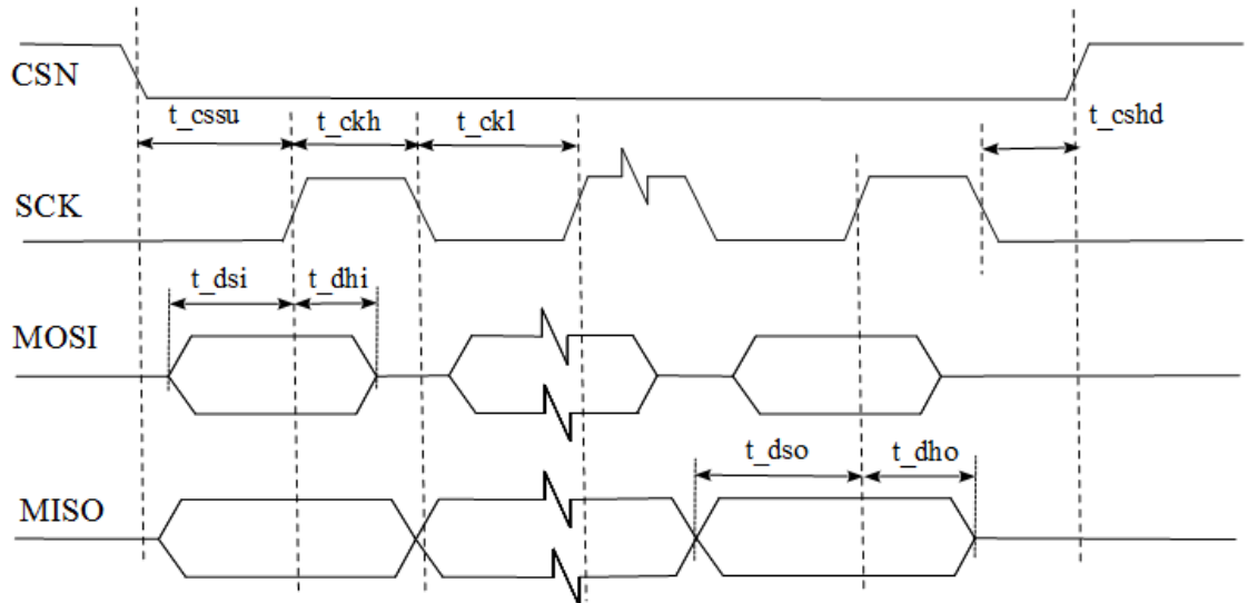
Figure 9: SPI Timing
