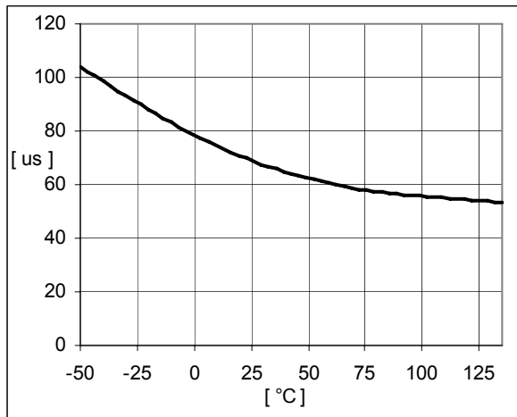
Fig. 10 Propagation Time t_{\text{PHL}} vs. Temperature
