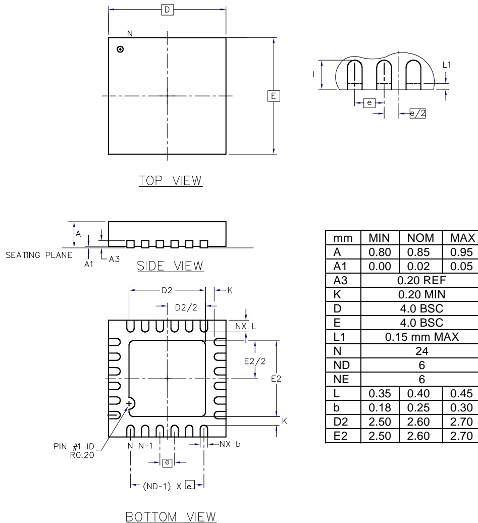
Figure 6.1: Package information
