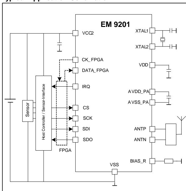
Typical Application Schematic
